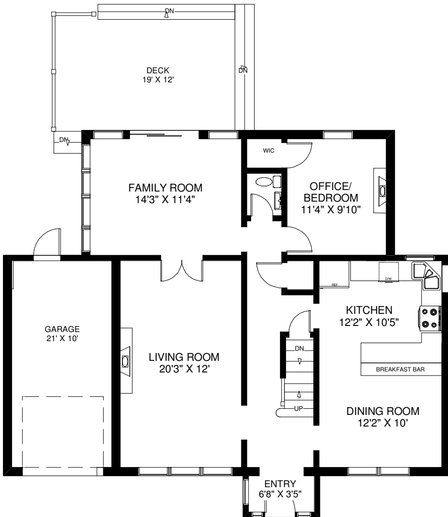
MAIN FLOOR APPROXIMATELY 1,150 SQ FT
