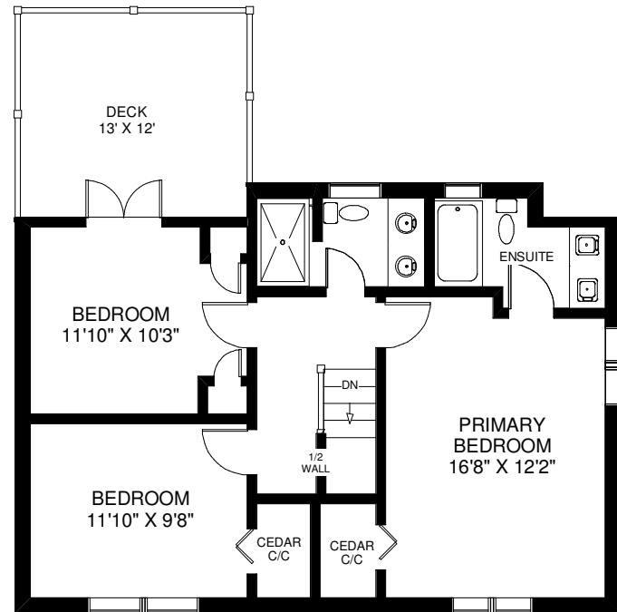
SECOND FLOOR APPROXIMATELY 760 SQ FT
