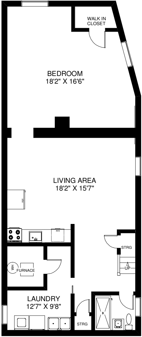
LOWER FLOOR APPROXIMATELY 1,060 SQ FT
