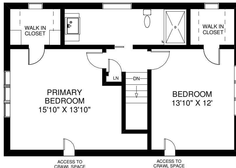
SECOND FLOOR APPROXIMATELY 670 SQ FT
