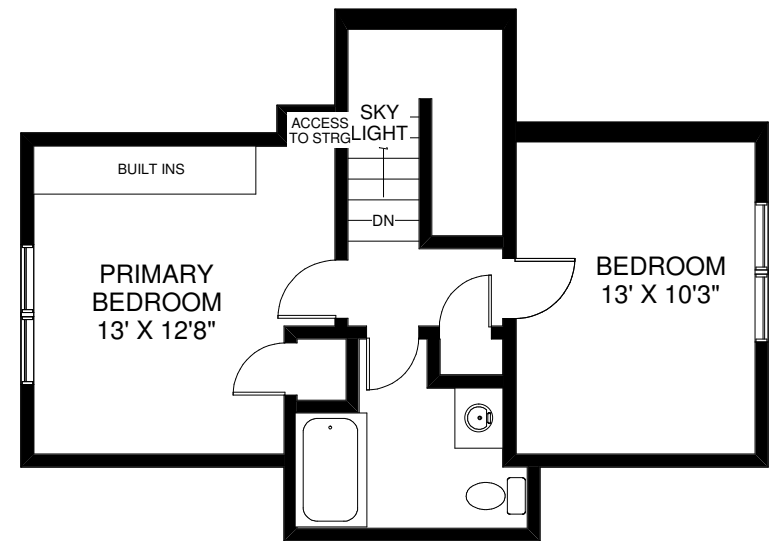
SECOND FLOOR APPROXIMATELY 500 SQ FT
