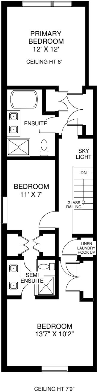
SECOND FLOOR APPROXIMATELY 800 SQ FT
