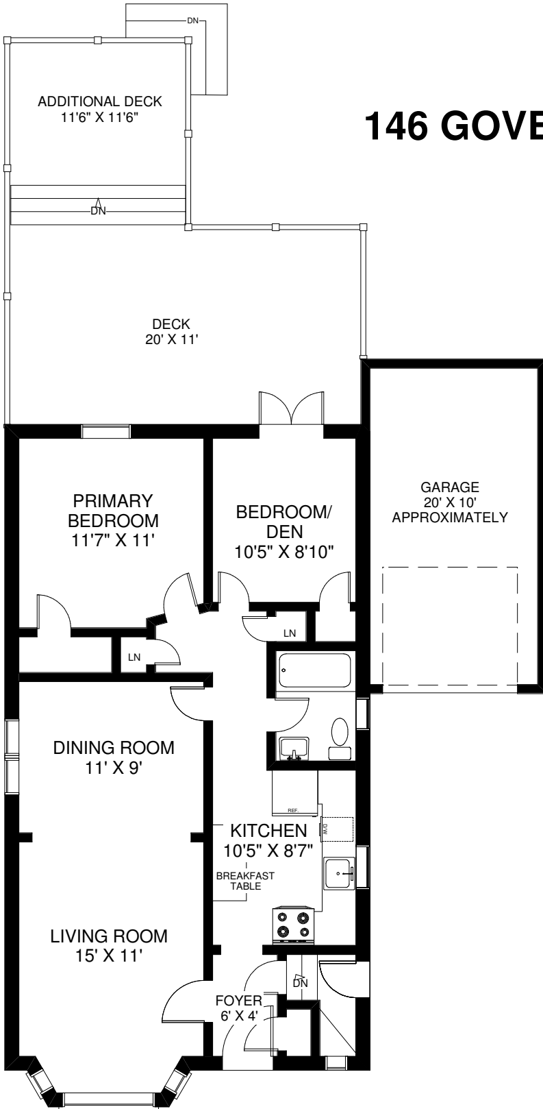
CEILING HT 8' MAIN FLOOR APPROXIMATELY 850 SQ FT
