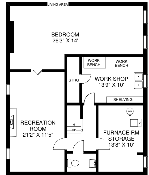
CEILING HT 6'9" LOWER FLOOR APPROXIMATELY 1,140 SQ FT
