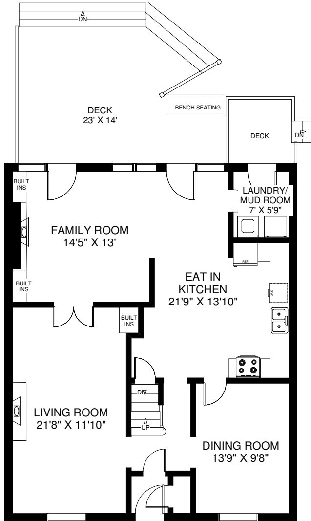
CEILING HT 8'2" MAIN FLOOR APPROXIMATELY 1,140 SQ FT
